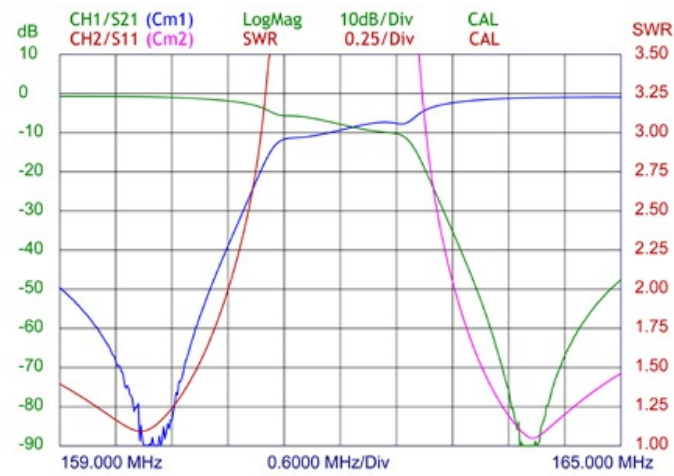
TYPICAL RESPONSE CURVE @ 5 MHZ DUPLEX SPACING
