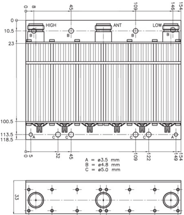
MOUNTING DETAILS
